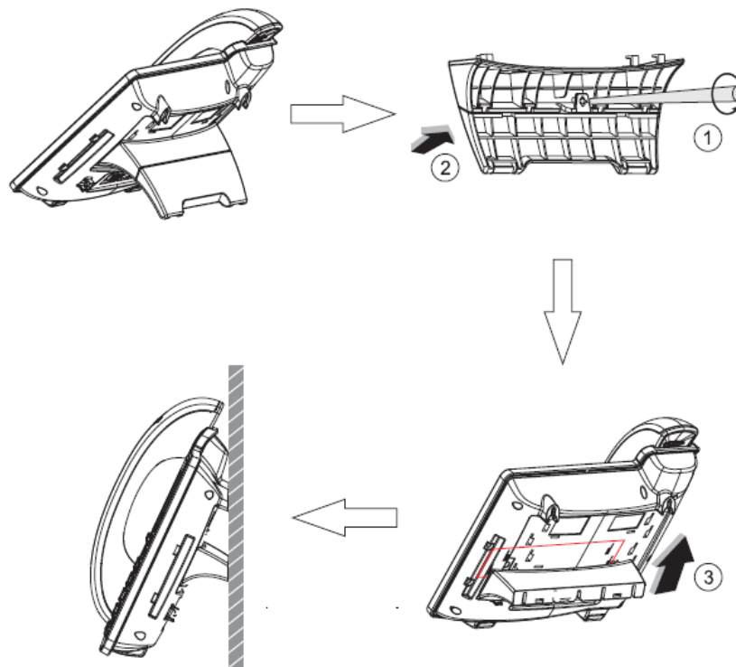
Figure 2 - Wall-mount Installation
