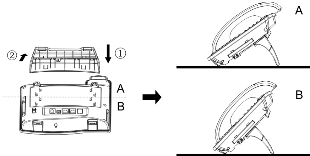
Figure 1 - Desktop Installation
